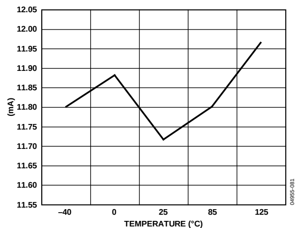
Figure 40. Current Consumption vs. Temperature @ CD = 3
