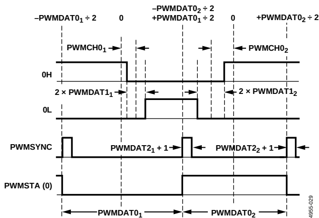
Figure 70. Typical PWM Outputs of the 3-Phase Timing Unit (Double Update Mode)
