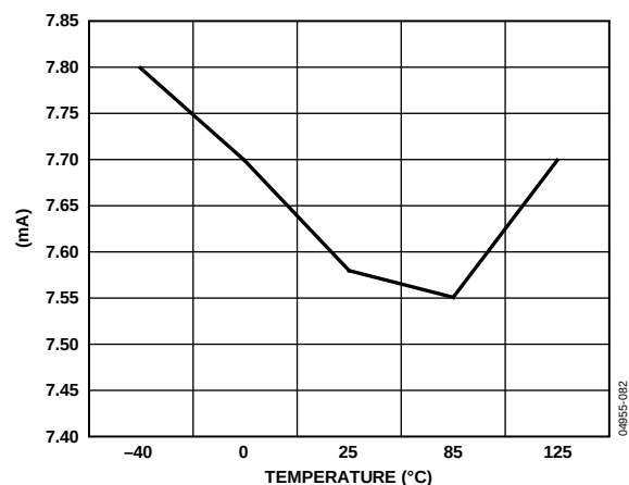
Figure 41. Current Consumption vs. Temperature @ CD = 7
