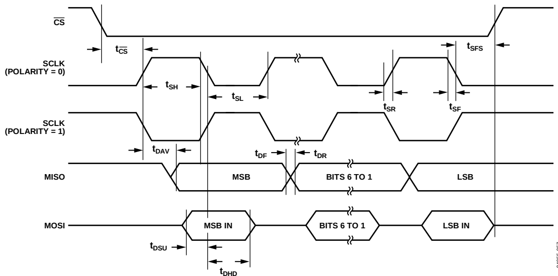
Figure 17. SPI Slave Mode Timing (Phase Mode = 1)
