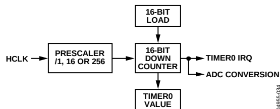
Figure 77. Timer0 Block Diagram
