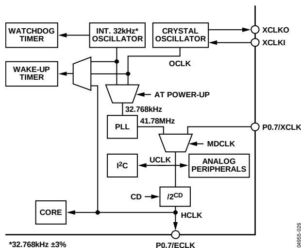
Figure 67. Clocking System
