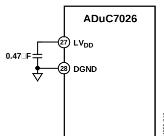
Figure 90. Voltage Regulator Connections
