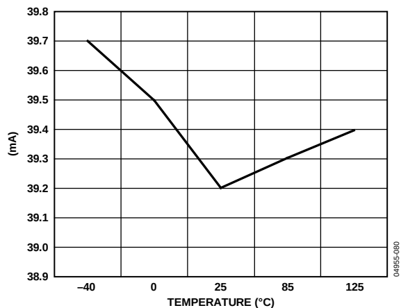
Figure 39. Current Consumption vs. Temperature @ CD = 0
