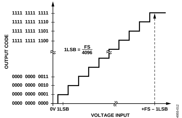
Figure 49. ADC Transfer Function in Pseudo Differential or Single-Ended Mode
