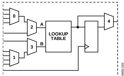
Figure 76. PLA Element
