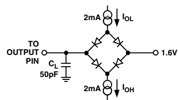
Figure 1. Load Circuit for Digital Output (SDO) Timing Specifications
