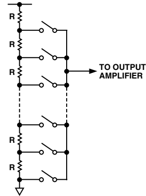
Figure 6. Resistor String
