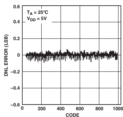
TPC 5. AD5313 Typical DNL Plot
