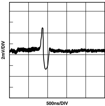
TPC 21. DAC-DAC Crosstalk
