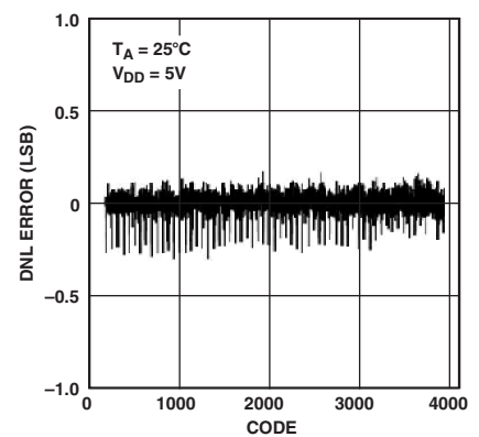
TPC 6. AD5323 Typical DNL Plot
