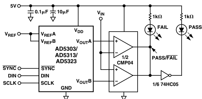
Figure 20. Window Detector Using AD5303/AD5313/AD5323
