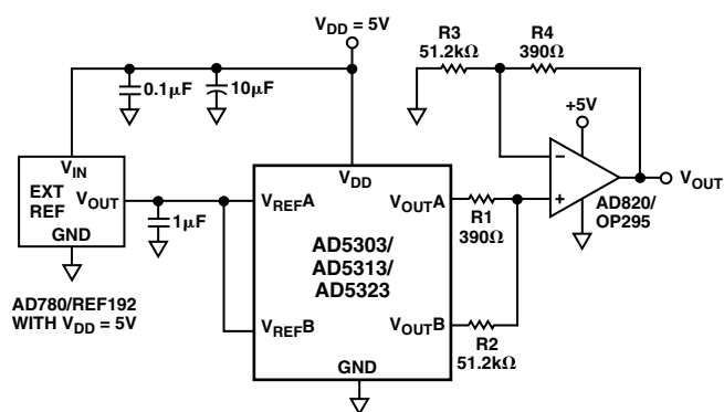
Figure 21. Coarse/Fine Adjustment
