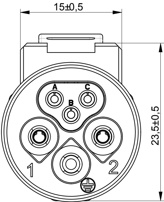
MATING FACE
