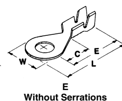
E Without Serrations
