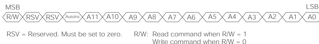
Figure 3-15: Command Word Format
