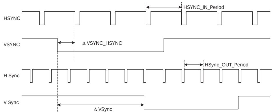
Figure 3-1: HD-SD Calculation
