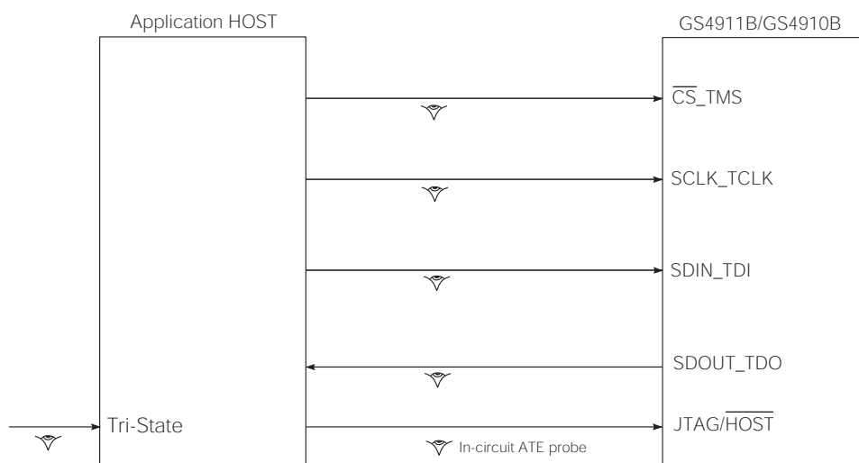
Figure 3-20: System JTAG
