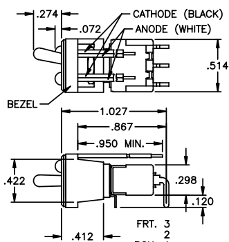
J95—TWO LED's
