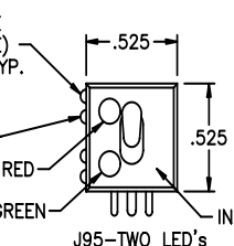
J95—TWO LED's
