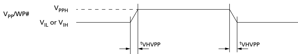
Figure 26: Accelerated Program AC Timing
