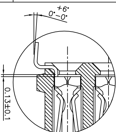
DETAIL A SCALE 20:1
