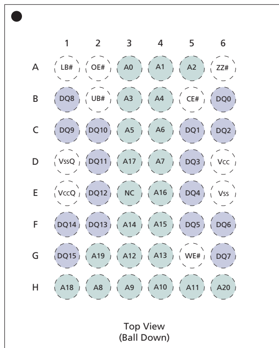
Figure 1: Ball Assignment – 48-Ball VFBGA
