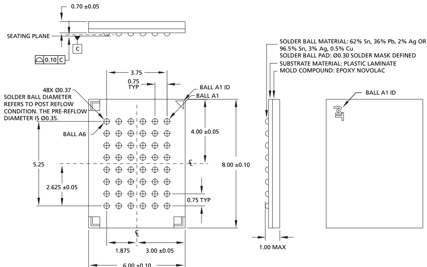
Figure 25: 48-Ball VFBGA
