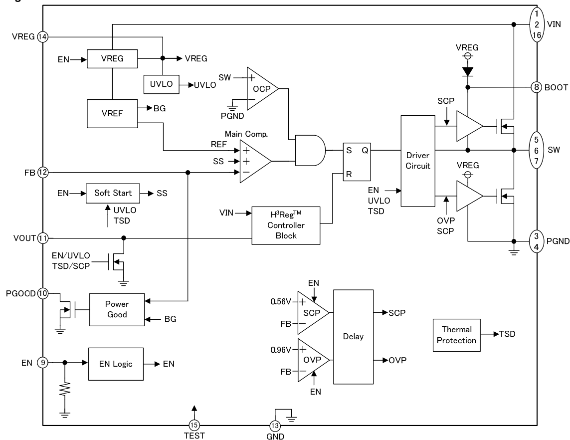
Figure 3. Block Diagram
