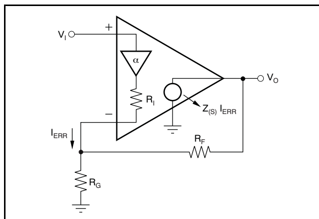
Figure 76. Current-Feedback Transfer Function Analysis Circuit
