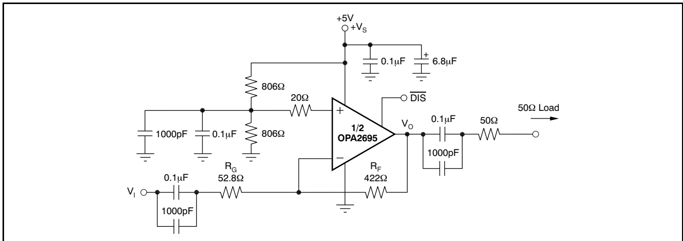
Figure 71. AC-Coupled, G = -8\text{V/V} , Single-Supply Specifications and Test Circuit
