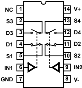
HS1-303ARH, HS-303BRH (SBDIP), CDIP2-T14 TOP VIEW
