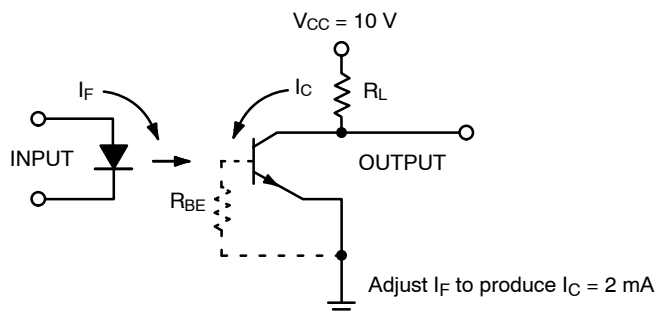
Figure 11. Switching Time Test Circuit and Waveform
