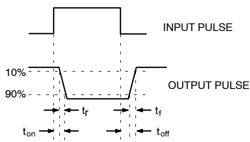
Figure 11. Switching Time Test Circuit and Waveform
