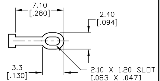
TERMINATION DETAIL
