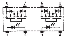
Terminal Arrangement/ Internal Connections (Top View)
