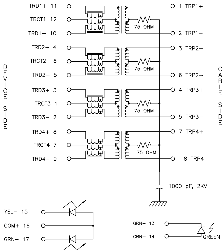
SCHMATIC
