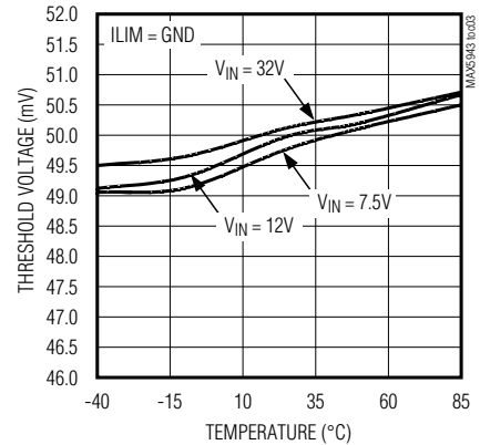
CURRENT-LIMIT/CIRCUIT-BREAKER THRESHOLD VOLTAGE vs. TEMPERATURE
