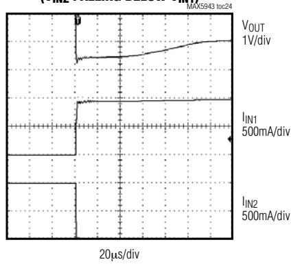
ORing SWITCHOVER WAVEFORM ( V_{IN2} FALLING BELOW V_{IN1} )
