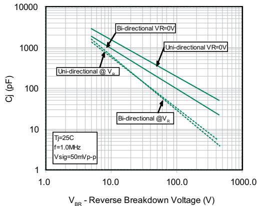
Figure 5 - Typical Junction Capacitance Uni-Directional
