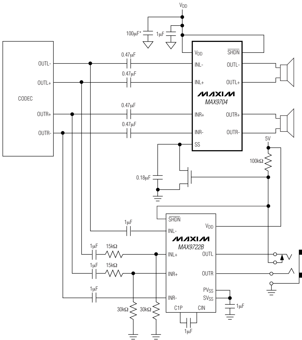
System Diagram
