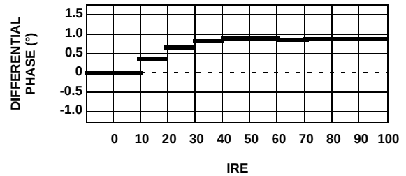
FIGURE 36. DIFFERENTIAL PHASE
