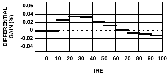
FIGURE 35. DIFFERENTIAL GAIN
