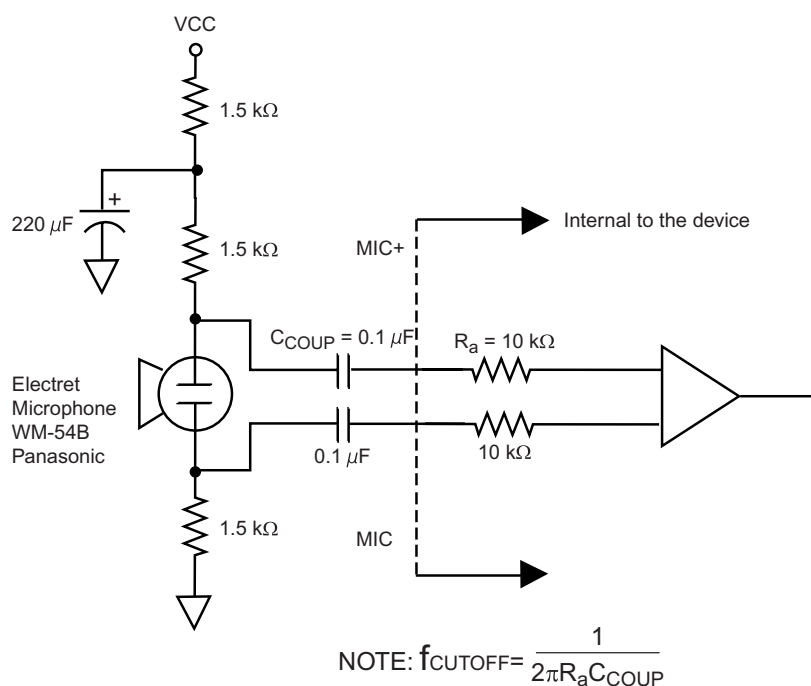
Figure 1: Microphone Input
