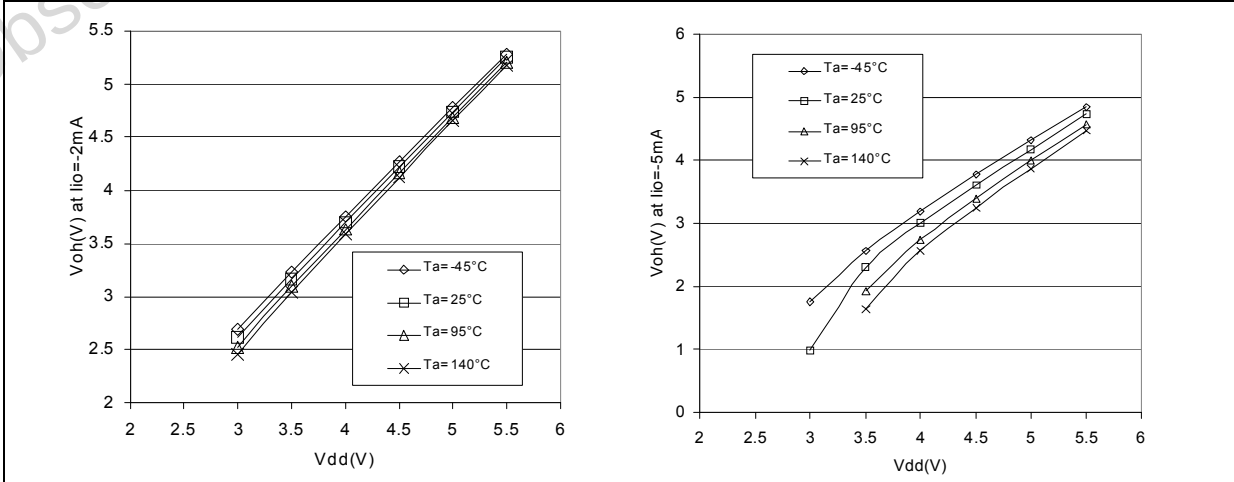
Figure 86. Typical V_{DD} - V_{OH} versus V_{DD}
