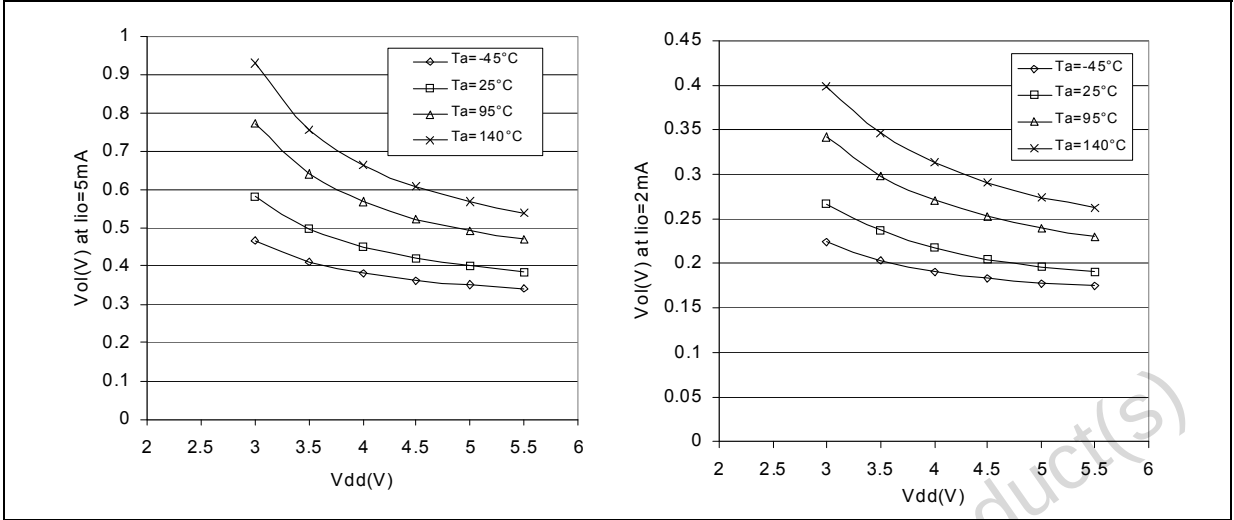
Figure 84. Typical V_{OL} versus V_{DD} (standard)
