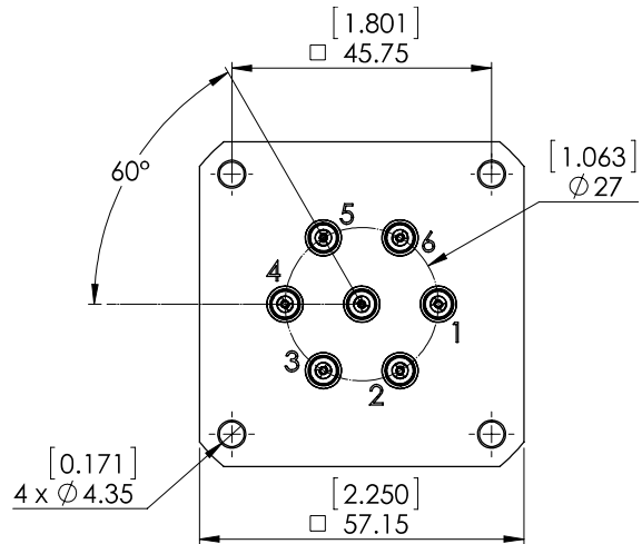
SMA 2.9 Connectors
