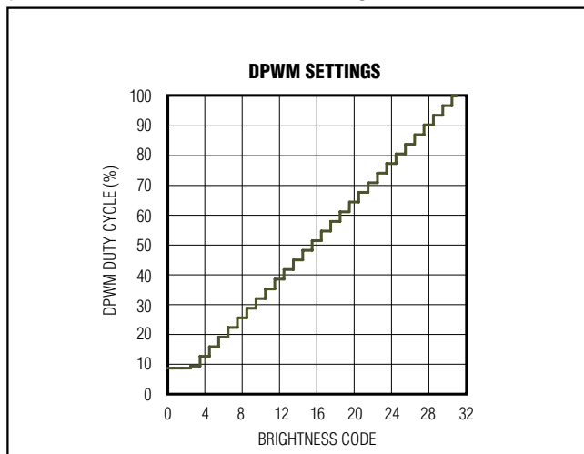
Figure 3. DPWM Settings
