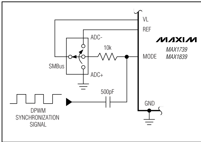
Figure 6. DPWM Synchronization
