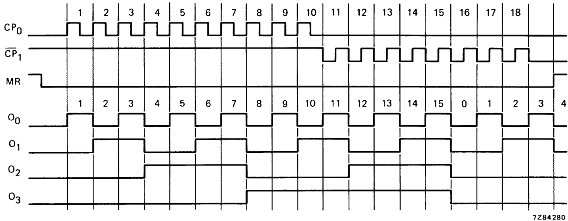
Fig.6 Timing diagram.
