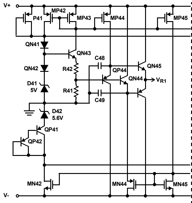
TTL/CMOS REFERENCE CIRCUIT
