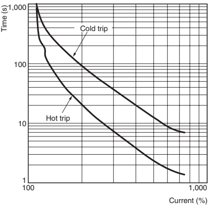
Trip Class 10
