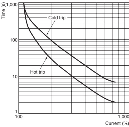
Trip Class 15
