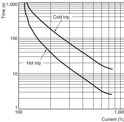
Trip Class 20
