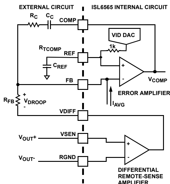
FIGURE 7. OUTPUT VOLTAGE AND LOAD-LINE REGULATION WITH OFFSET ADJUSTMENT
