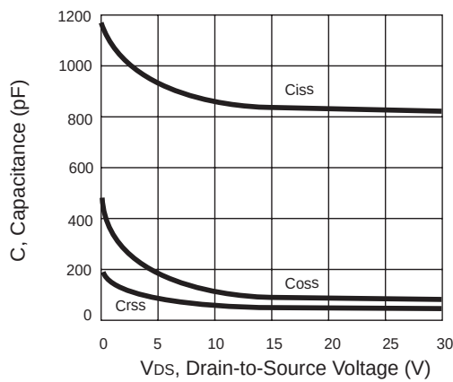
Figure 3. Capacitance
