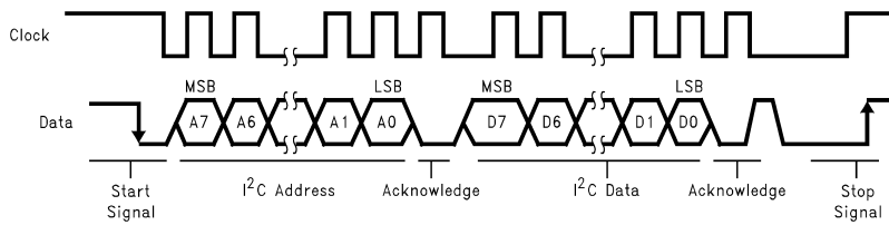
Figure 53. I²C Bus Format
