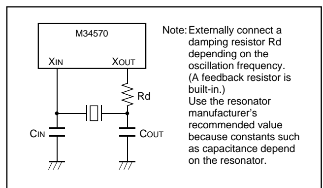
Fig. 33 Ceramic resonator external circuit
