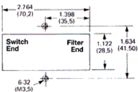
PM90 Screw-Mount Series
