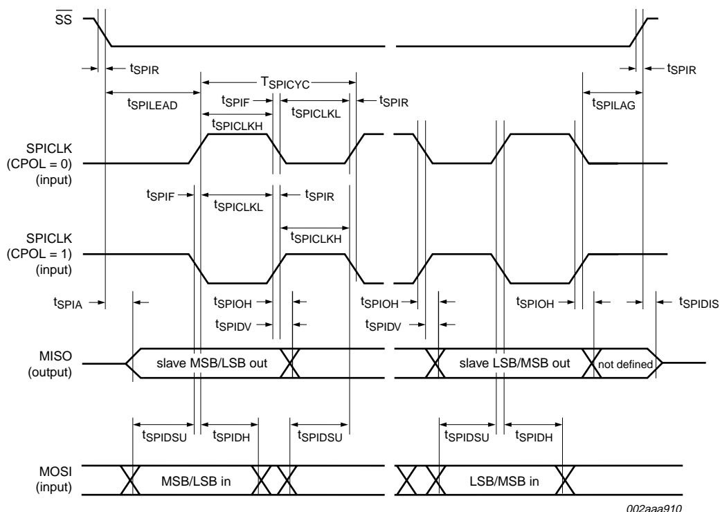
Fig 28. SPI slave timing (CPHA = 0)
