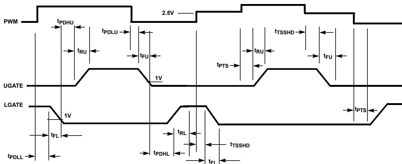
FIGURE 3. TIMING DIAGRAM
