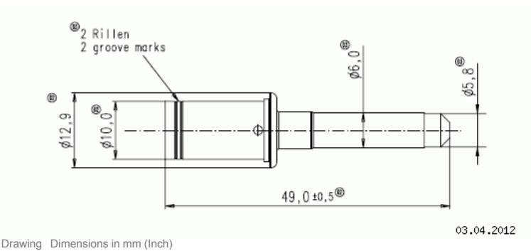
Drawing Dimensions in mm (Inch)
