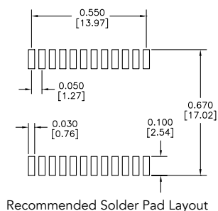
Recommended Solder Pad Layout
