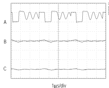
LIGHT-LOAD, PWM-MODE SWITCHING WAVEFORMS
