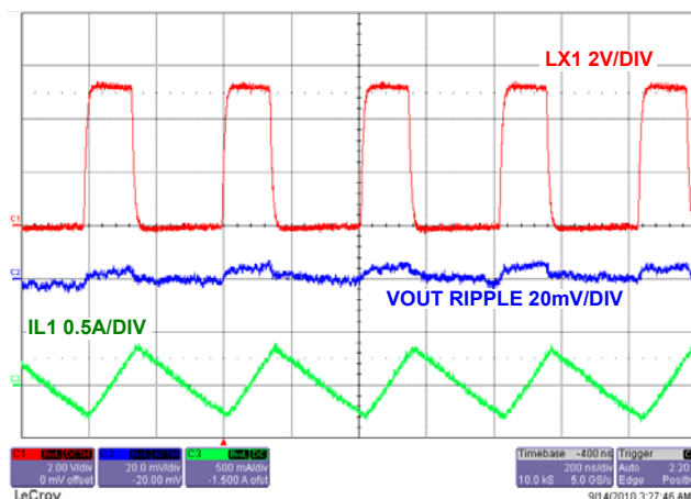
FIGURE 36. STEADY STATE OPERATION AT NO LOAD CHANNEL 1
