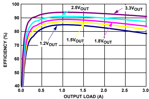
FIGURE 32. EFFICIENCY vs LOAD, 5V IN DUAL CHANNEL 1, T_A = +25^\circ C
