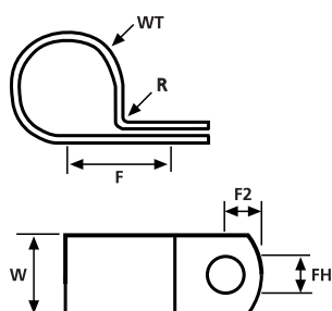
Aluminium P Clips
