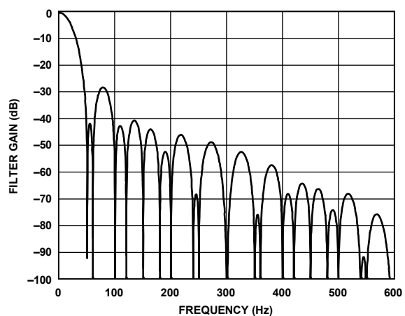
Figure 46. 27.27 SPS ODR, 36.67 ms Settling Time
