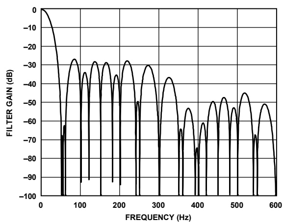
Figure 47. 25 SPS ODR, 40 ms Settling Time
