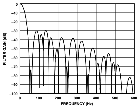
Figure 48. 20 SPS ODR, 50 ms Settling Time
