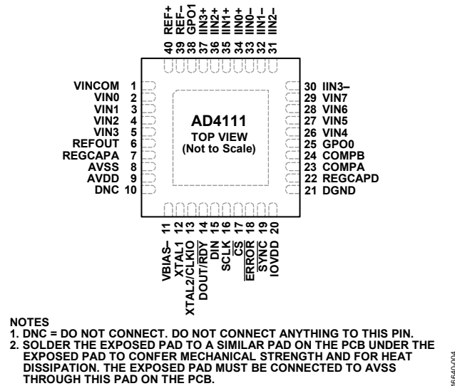
Figure 4. Pin Configuration
