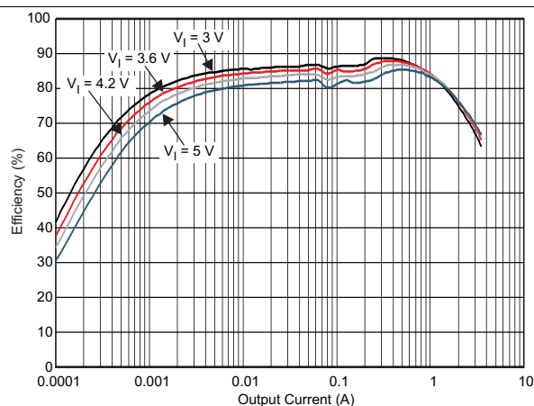
DCDC4 V_O = 1.1375 V PFM Mode DEF25012-1 \mu H 25°C
