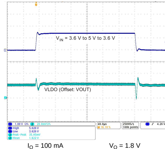
Figure 8-19. Line Transient Response LDO6, LDO8
