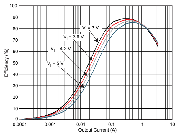
DCDC4 V_O = 1.1375 V PFM Mode DEF322512-1 \mu H 25°C
