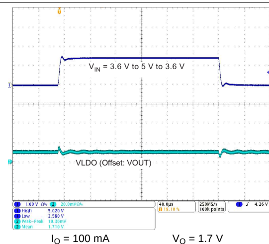
Figure 8-15. Line Transient Response LDO4, LDO5
