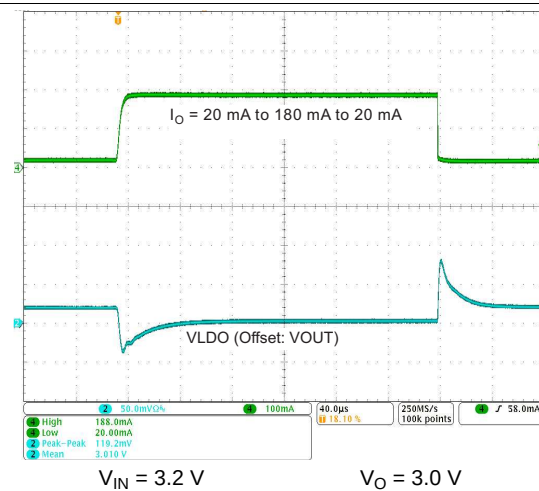
Figure 8-21. Load Transient Response LDO7
