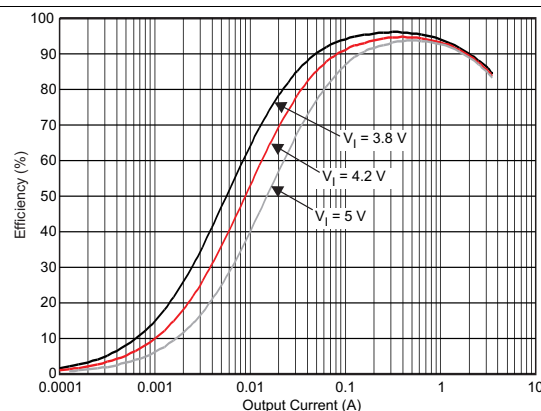
DCDC4 V_O = 3.3 V PWM Mode DEF322512-1 \mu H 25°C
