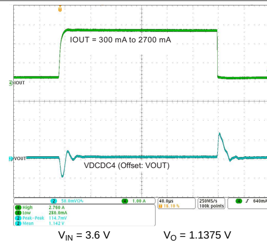
Figure 8-5. Load Transient Response DCDC4
