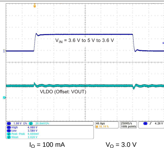
Figure 8-16. Line Transient Response LDO4, LDO5
