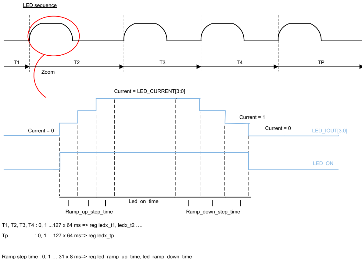
Figure 7-29. LED Sequencer
