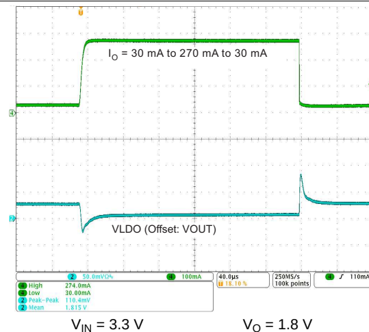
Figure 8-23. Load Transient Response LDO10
