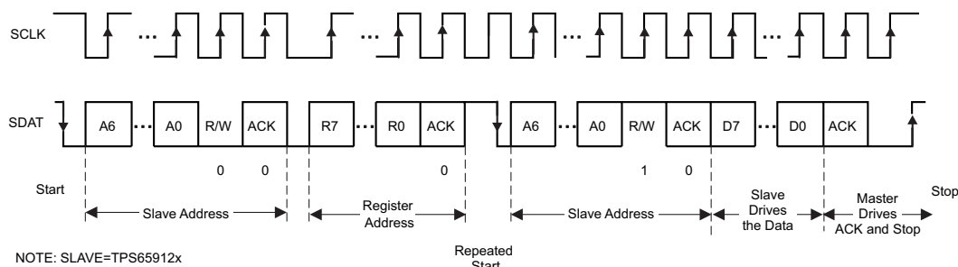
Figure 7-25. I 2 C Interface READ from TPS65912x; F/S mode
