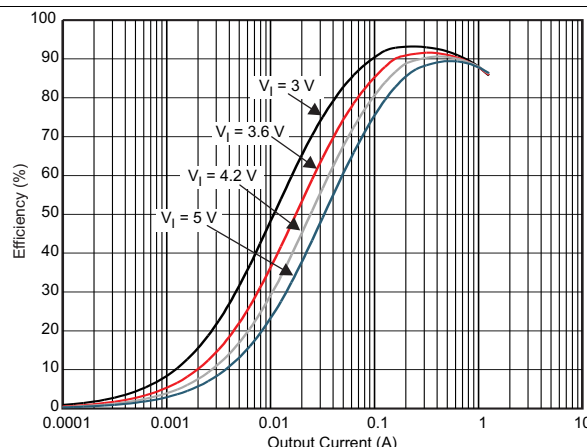
DCDC2 V_O = 2.25 V VLS201612-1 \mu H PFM Mode 25°C
