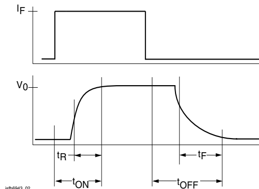
Fig. 2 Switching Waveform
