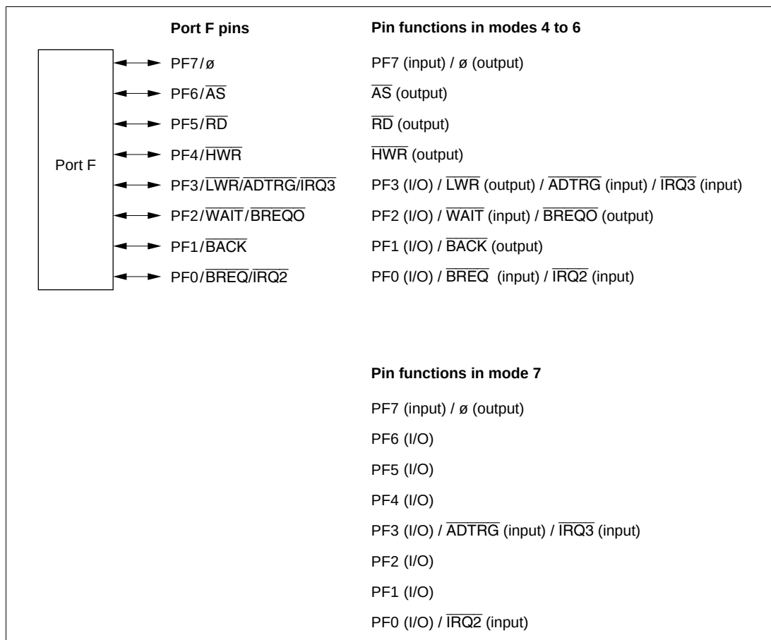
Figure 10B-22 Port F Pin Functions
