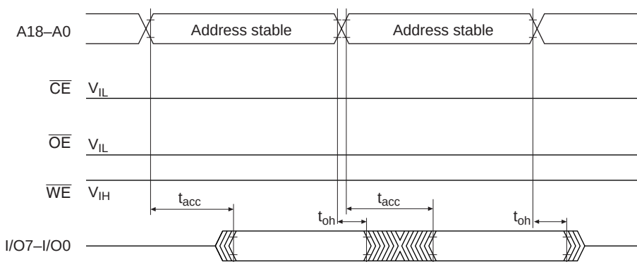
Figure 22-21 \overline{\text{CE}} and \overline{\text{OE}} Enable State Read Timing Waveforms
