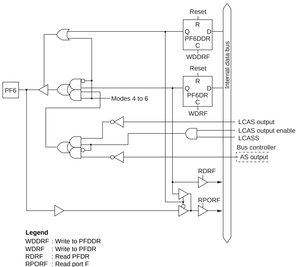
Figure C-11 (g) Port F Block Diagram (Pin PF6)
