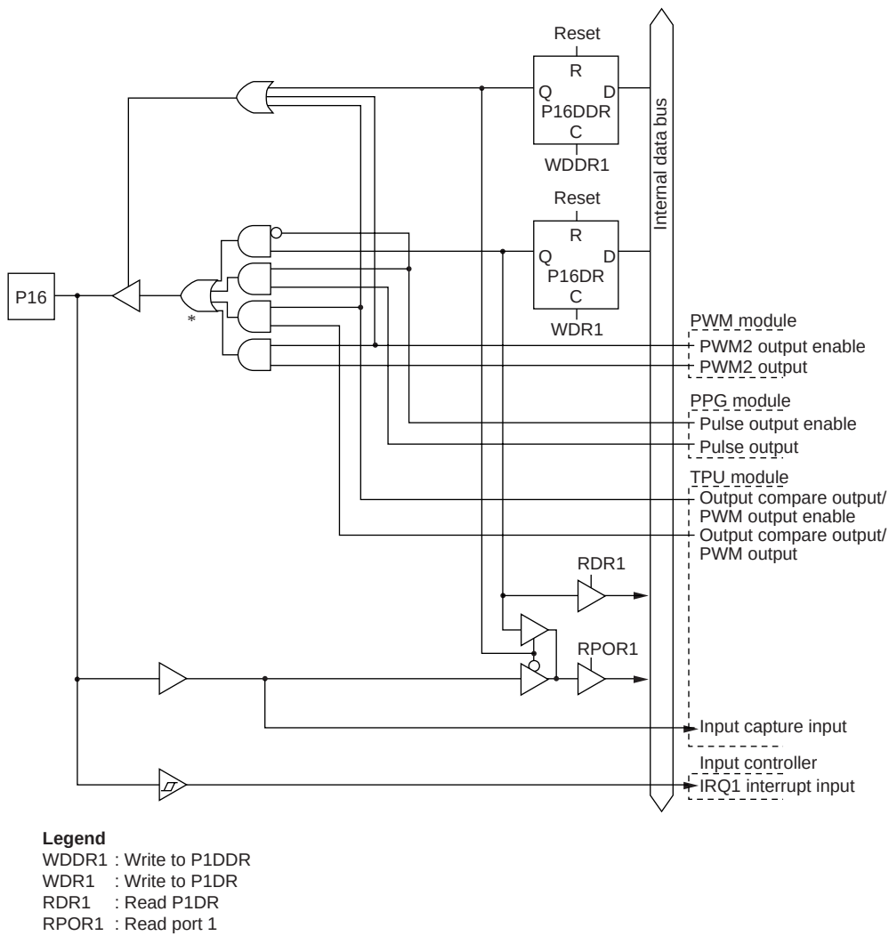
Figure C-1 (e) Port 1 Block Diagram (Pin P16)
