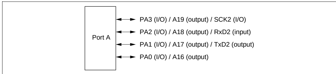
Figure 10A-7 Port A Pin Functions (Modes 4 to 6)
