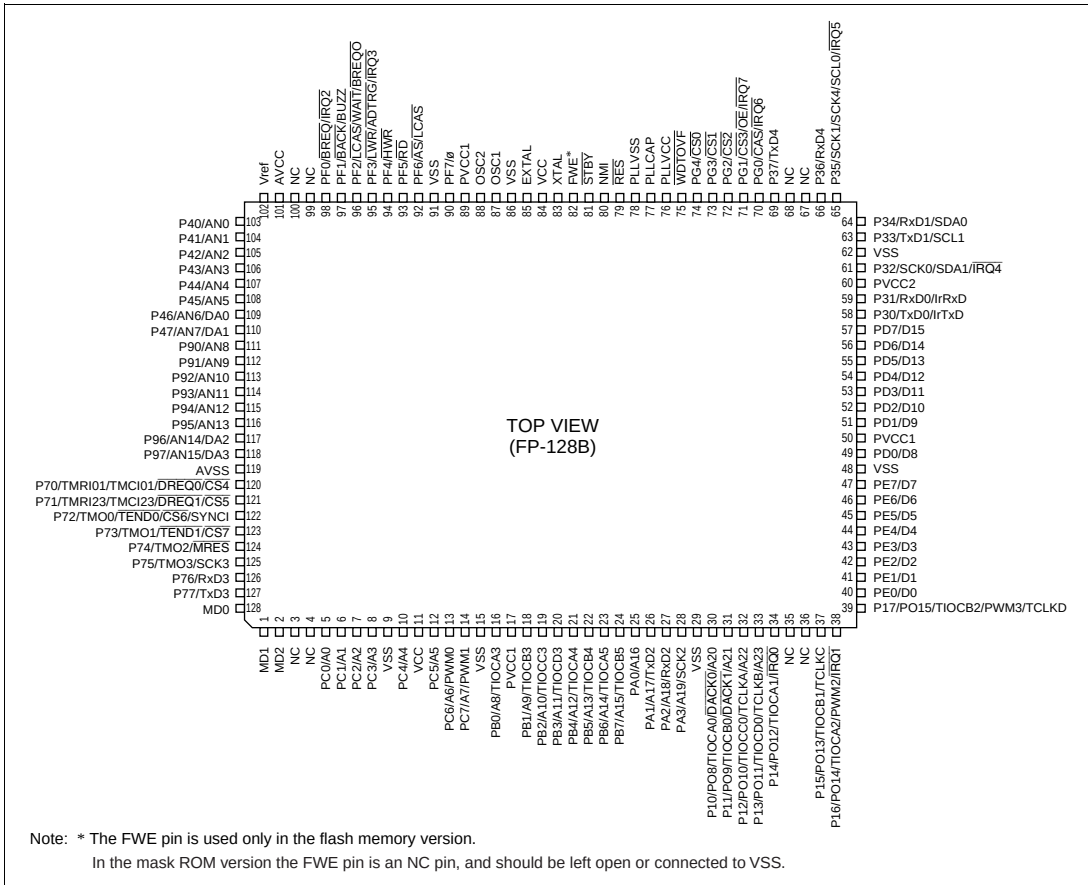
Figure 1-3 (a) H8S/2633, H8S/2632, H8S/2631, H8S/2633F Pin Arrangement (FP-128B: Top View)
