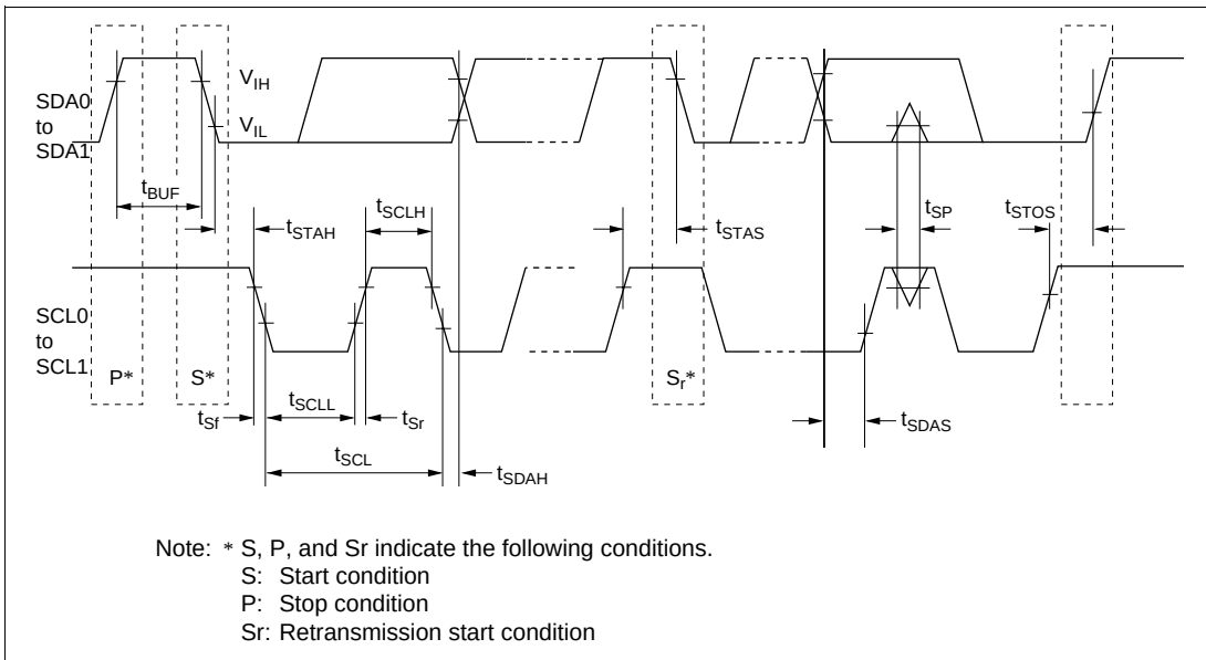
Figure 25-33 I²C Bus Interface Input/Output Timing (Option)
