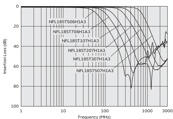
NFL18ST_H Series
