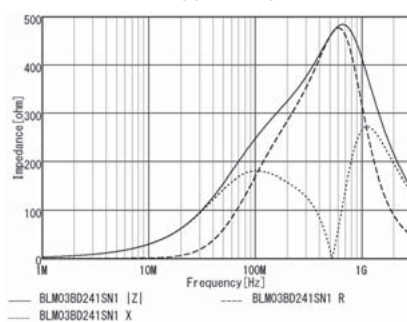
BLM03BD241SN1
