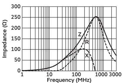
BLA31BD121SN4
