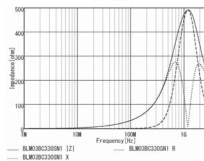
BLM03BC330SN1
