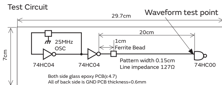
Comparison of Test Effect (25MHz)
