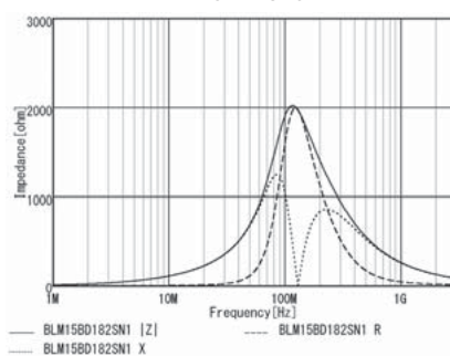
BLM15BD182SN1
