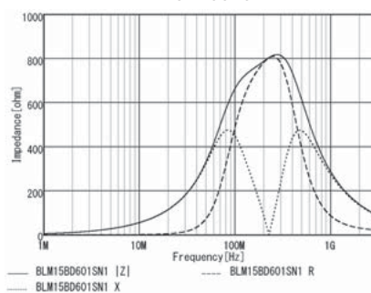
BLM15BD601SN1
