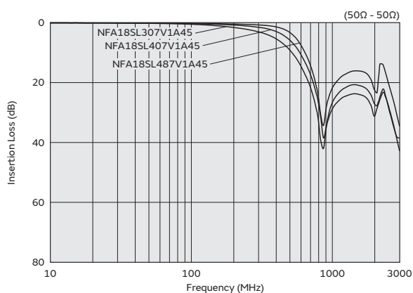
NFA18SL 307/407/487 V1A45
