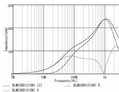
BLM03BD121SN1
