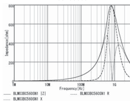
BLM03BC560SN1
