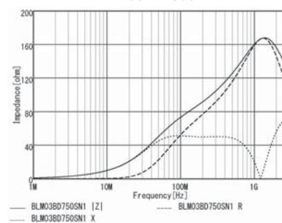
BLM03BD750SN1
