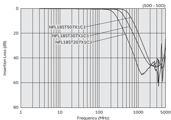
NFL18ST_X Series
