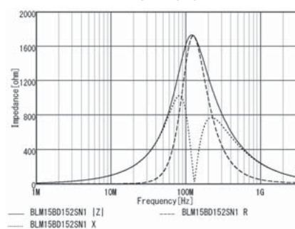
BLM15BD152SN1
