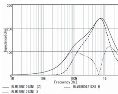
BLM15BD121SN1
