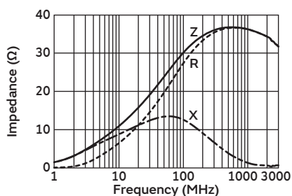
BLA31AG300SN4
