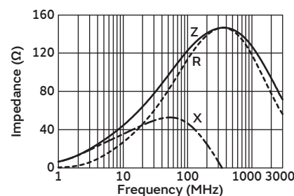
BLA31AG121SN4
