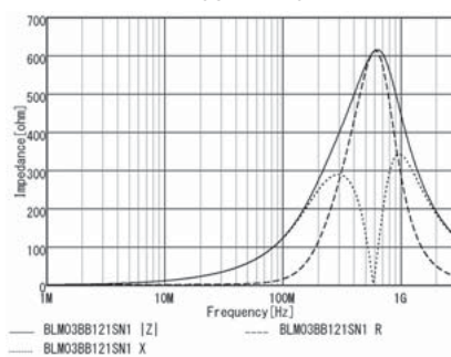
BLM03BB121SN1
