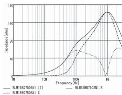
BLM15BD750SN1
