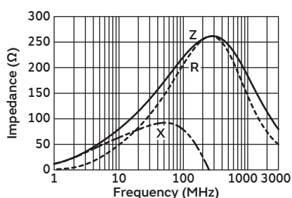
BLA31AG221SN4
