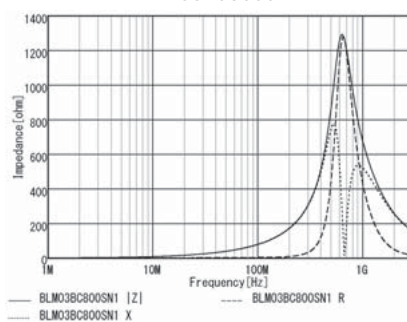
BLM03BC800SN1
