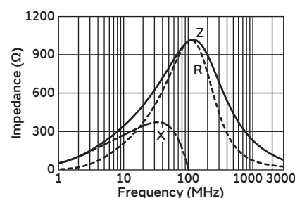
BLA31AG102SN4
