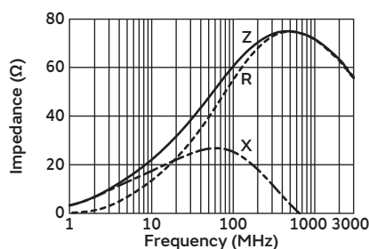
BLA31AG600SN4
