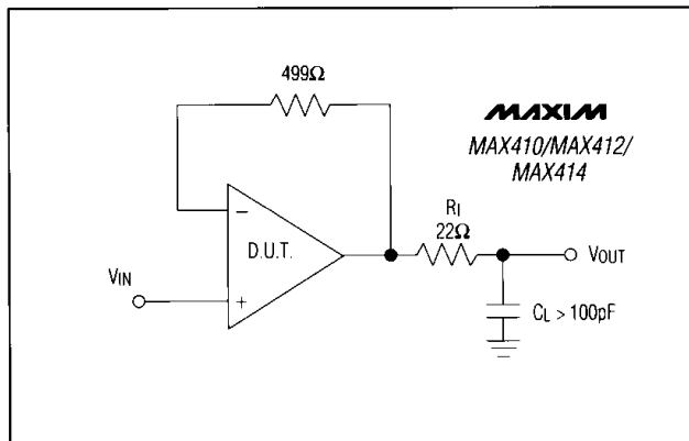
Figure 7a. Capacitive Load Driving Circuit
