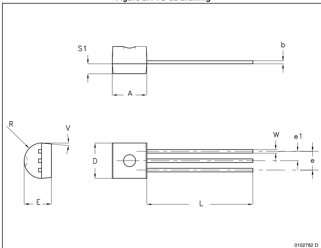
Figure 17. TO-92 drawing
