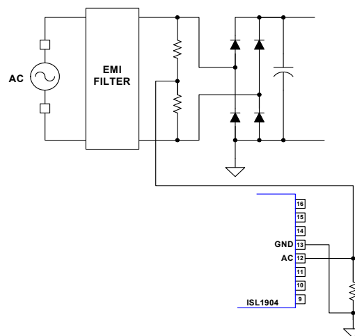
FIGURE 11. AC DETECTION
