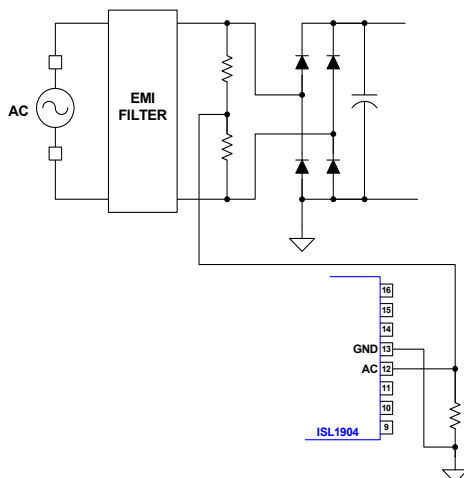
FIGURE 10. AC DETECTION
