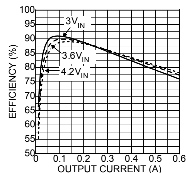
Efficiency 0.6V OUT
