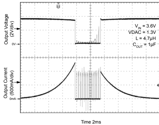
Current Limit Transient (Bypass Mode)
