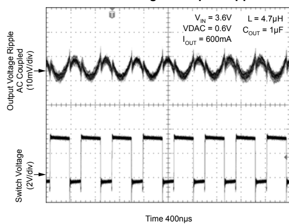
Switch Voltage - Output Ripple
