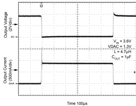
Current Limit Transient (PWM Mode)
