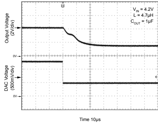
Bypass Mode Transient
