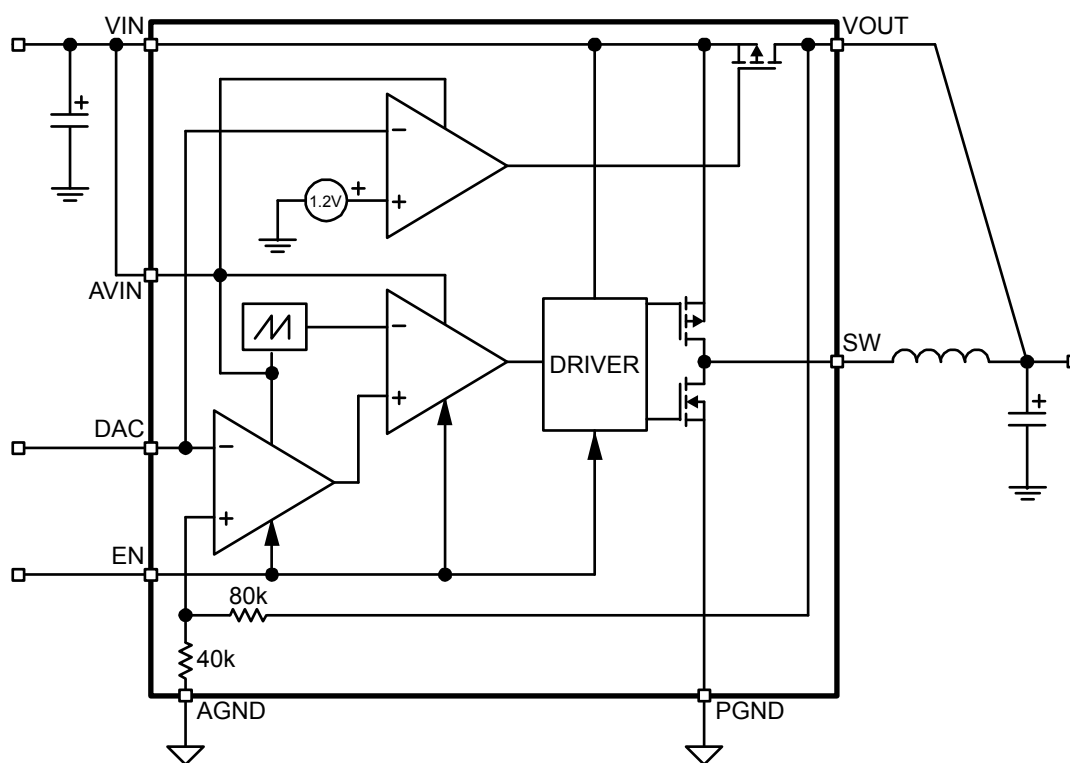
MIC2224 Block Diagram
