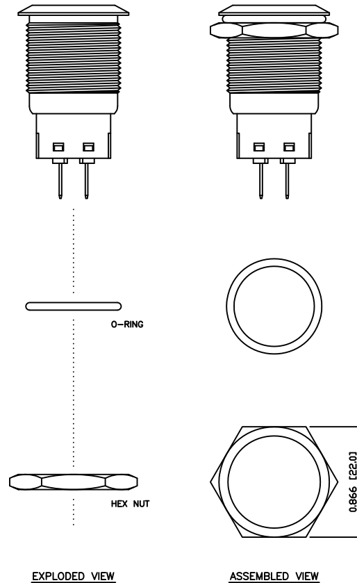
EXPLODED VIEW
