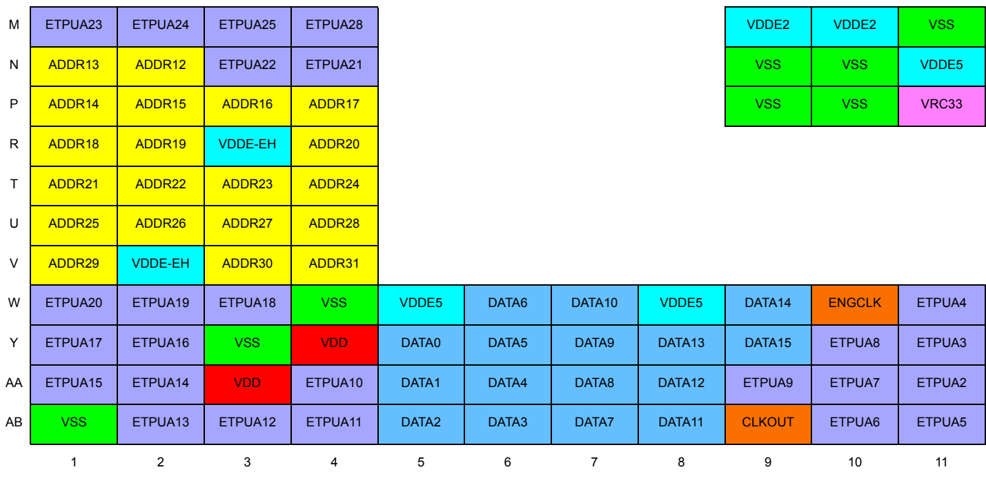
Figure 5. 324-pin TEPBGA package ballmap (southwest, viewed from above)
